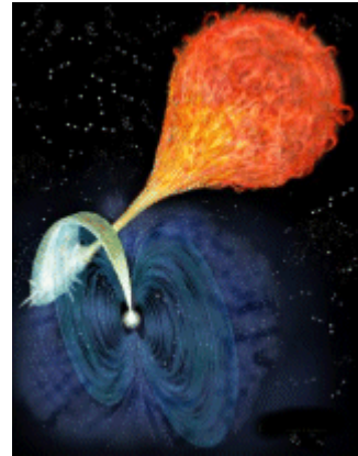
Artistic impression of an AM Her system. The blue haze represents the white dwarf's magnetosphere. Image copyright Russell Kightley Media
